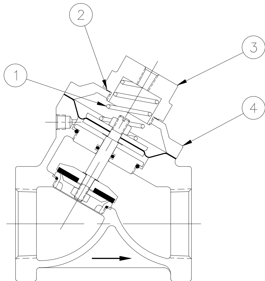
SERIES 424 NORMALLY OPEN VALVE
