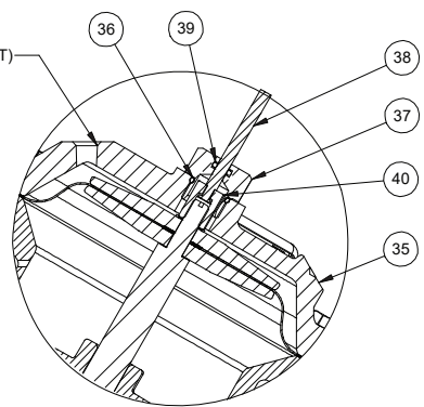
1073156 (V42K-3021-00000) POSITION INDICATOR
