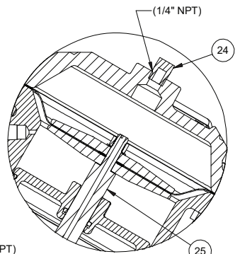
1073158 (V42K-3030-00000) NORMALLY CLOSED
