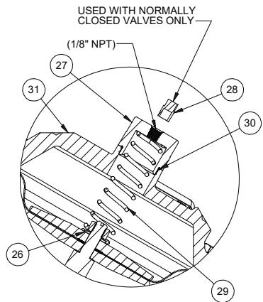
1073148 (V42K-3002-00000) SPRING ASSIST CLOSED
