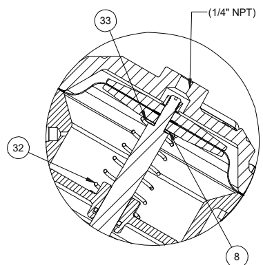
1073146 (V42K-3001-00000) SPRING ASSIST OPEN
