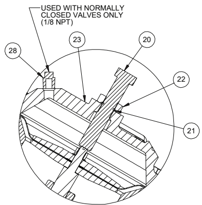
1073151 (V42K-3010-00000) LIMIT STOP
